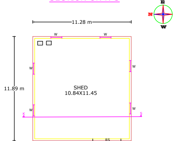
SECTION ON K-S
