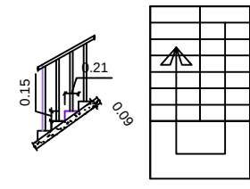
STAIRCASE DETAILS
