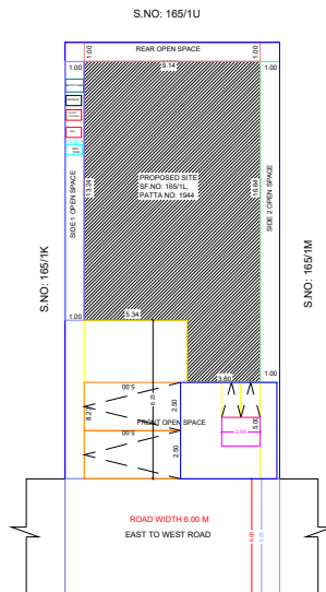
SITE PLAN
