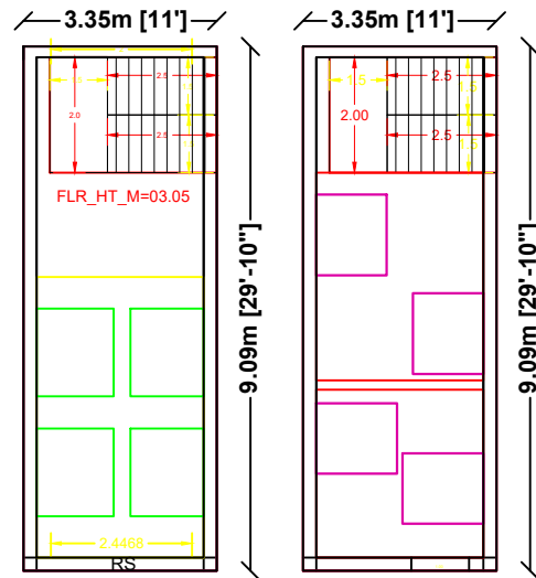
GROUND FLOOR PLAN (COMMERCIAL)
