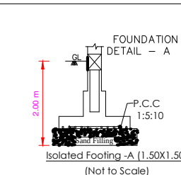
Foundation Detail - A (Not to Scale)
