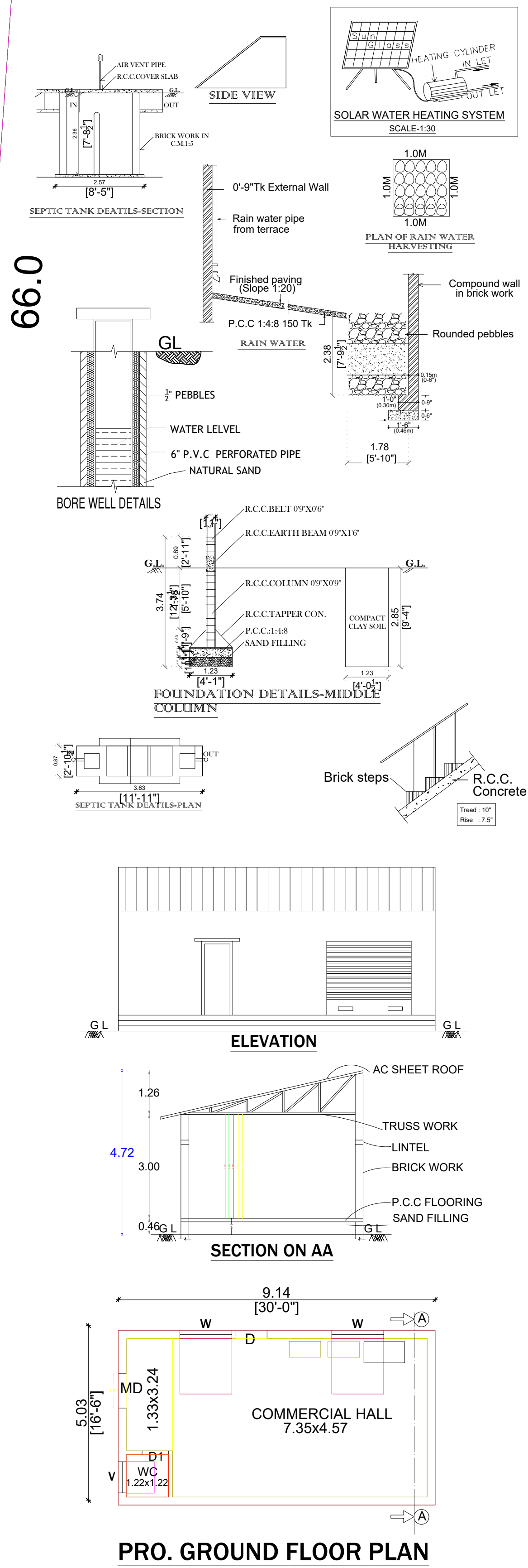
PRO. GROUND FLOOR PLAN
