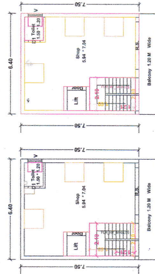
PLAN - Revised Ground Floor - Commercial
