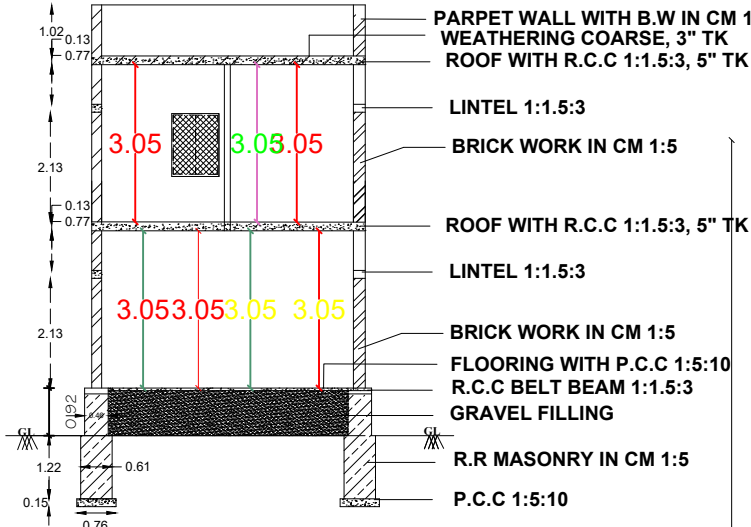
SECTION
