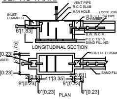
SEPTIC TANK:
