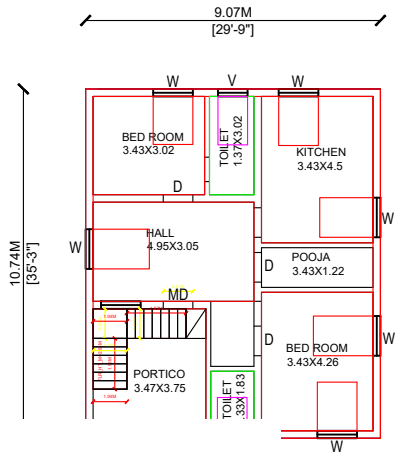
ND FLOOR
