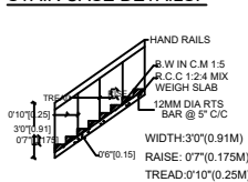
STAIR CASE DETAILS:-
