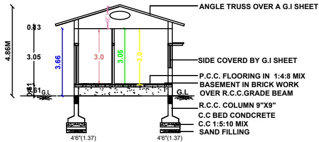
SECTION " AB "
