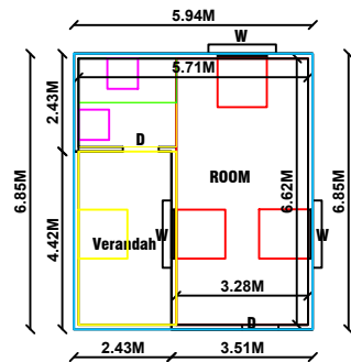
GROUND FLOOR PLAN ( G.I SHED )
