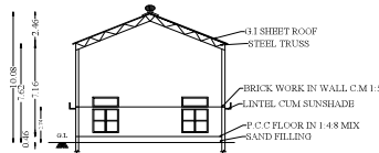
SECTION CD
