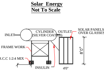
Waste Water Recycle Unit Not To Scale
