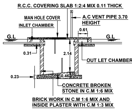
.SECTION ON SEPTIC TANK .
