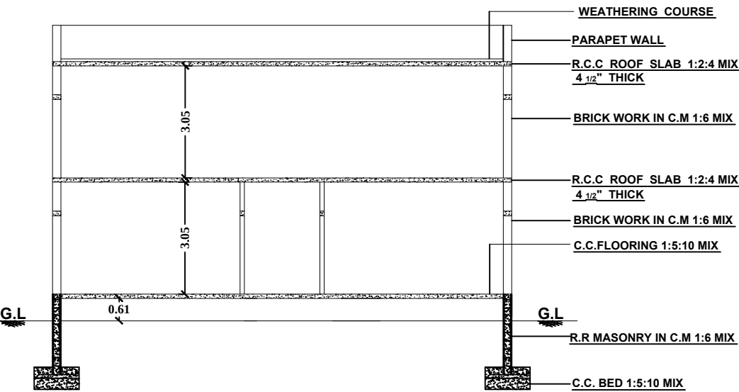
. SECTION ON "EF" .
