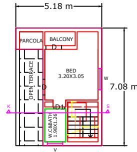
PROPOSED SECOND FLOOR PLAN
