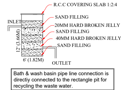
Waste Water Recycle Unit Not To Scale
