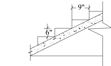
Staircase Detail Not To Scale
