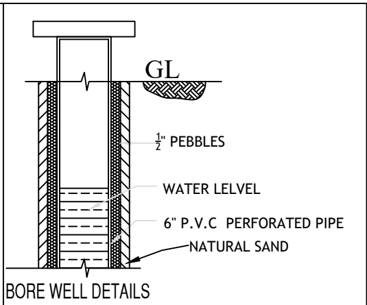
BORE WELL DETAILS
