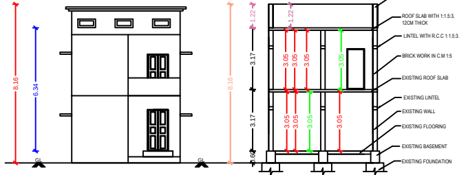
ELEVATION ( FACING EAST)
