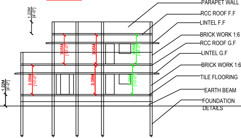
SECTION "A-B"
