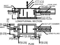
SEPTIC TANK:
