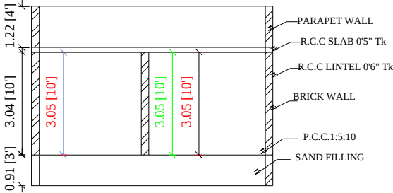
SECTION ON"AB"
