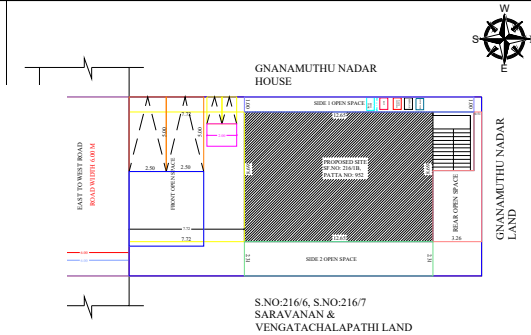
SITE PLAN
