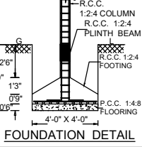
FOUNDATION DETAIL
