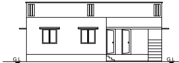
FRONT ELEVATION
