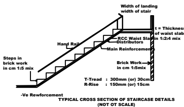
TYPICAL CROSS SECTION OF STAIRCASE DETAILS (NOT TO SCALE)
