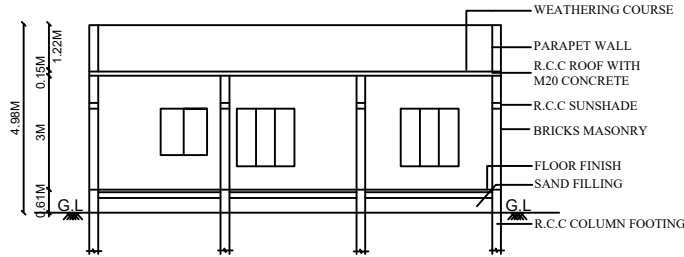
SECTION ON "SP"
