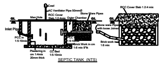
SEPTIC TANK (NTS)
