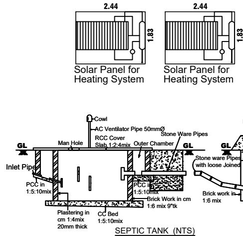
SEPTIC TANK (NTS)
