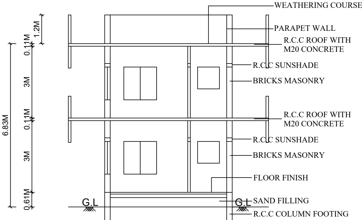
SECTION ON "SP"
