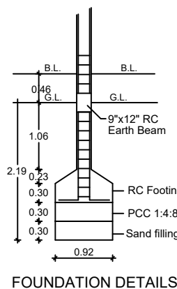
FOUNDATION DETAILS
