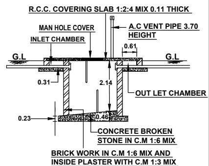
SECTION ON SEPTIC TANK
