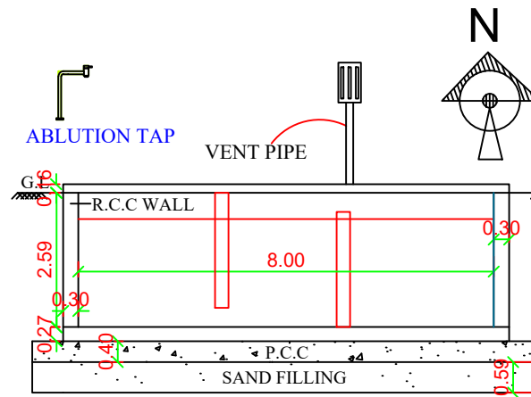
SECTION ON K-B
