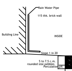
FOUNDATION DETAILS
