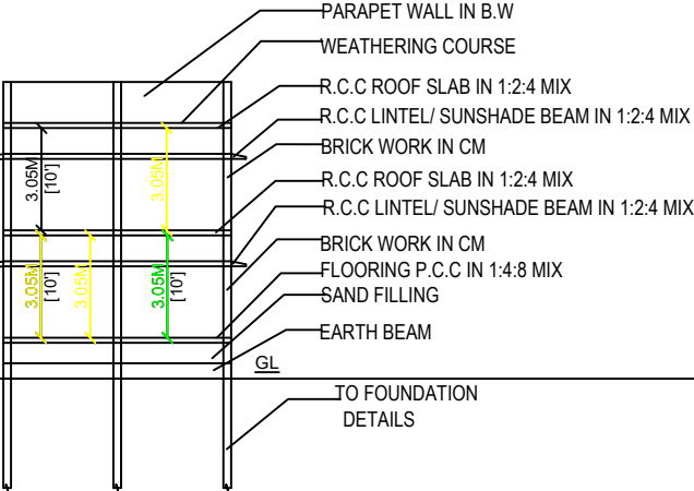
SECTION ON-AA
