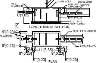
SEPTIC TANK:
