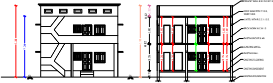
ELEVATION ( FACING NORTH )
