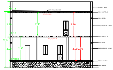
SECTION ON K-S
