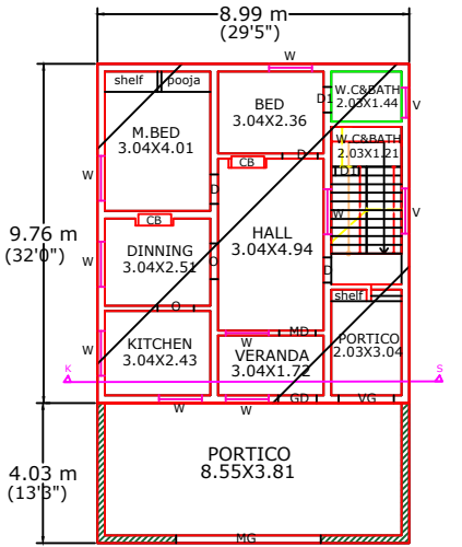
EXISTING GROUND FLOOR PLAN (Already Approved)
