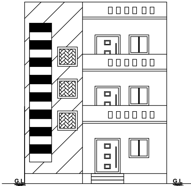
FRONT ELEVATION
