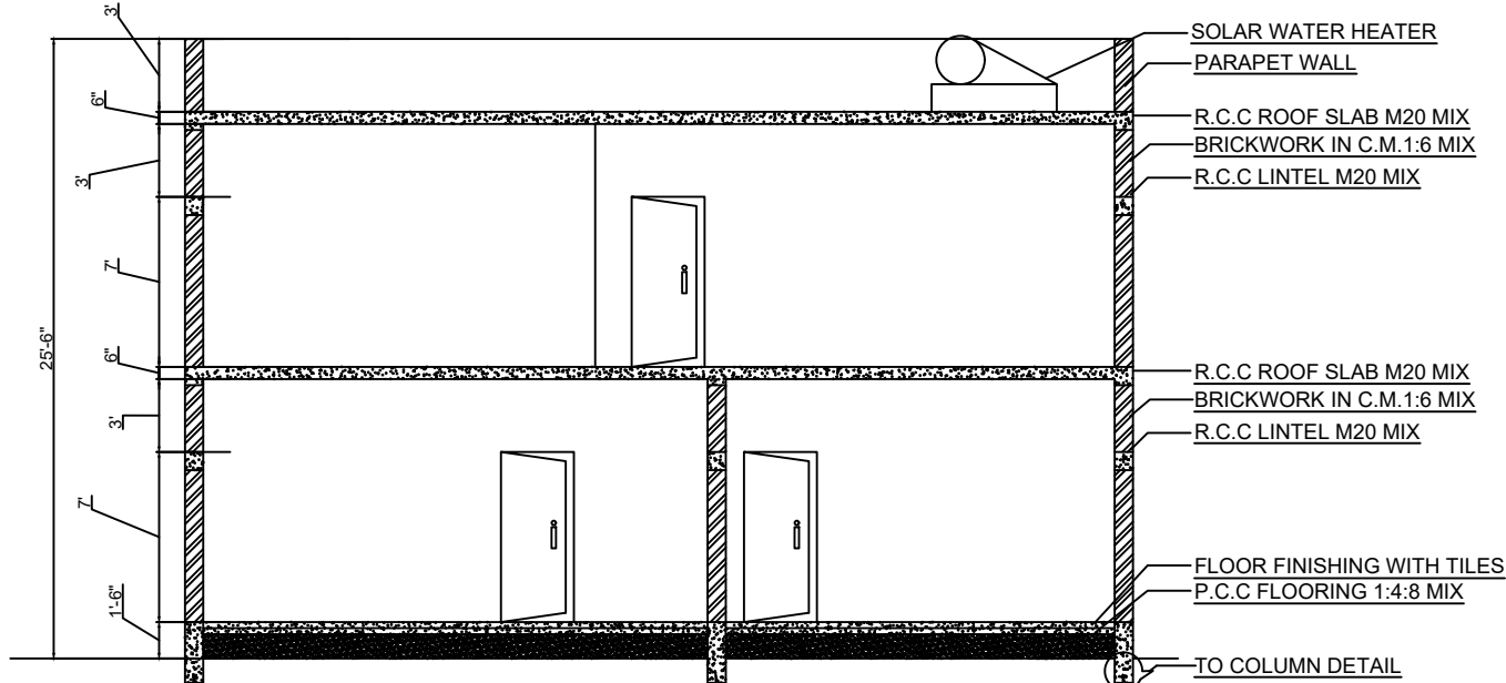
SECTIONA-B
