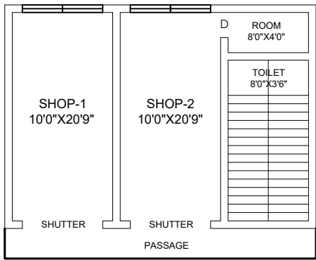
EXT. FIRST FLOOR PLAN [SOUTH FACING]
