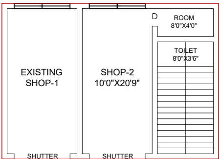
EXT. GROUND FLOOR PLAN [SOUTH FACING]
