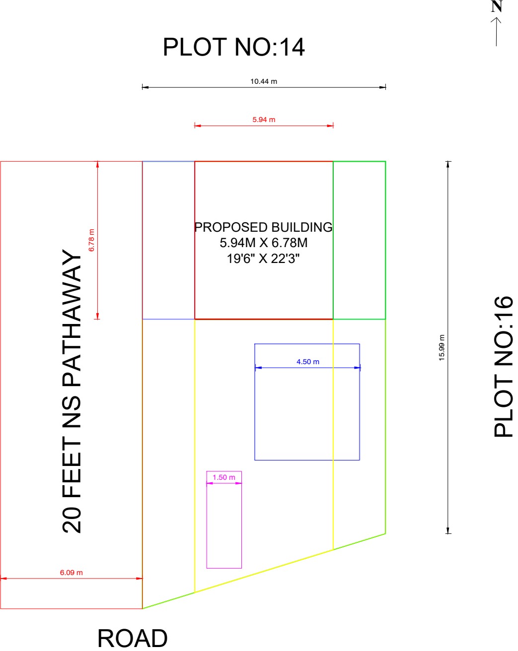
SITE PLAN
