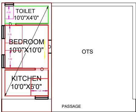
PRO. FIRST FLOOR PLAN [SOUTH FACING]
