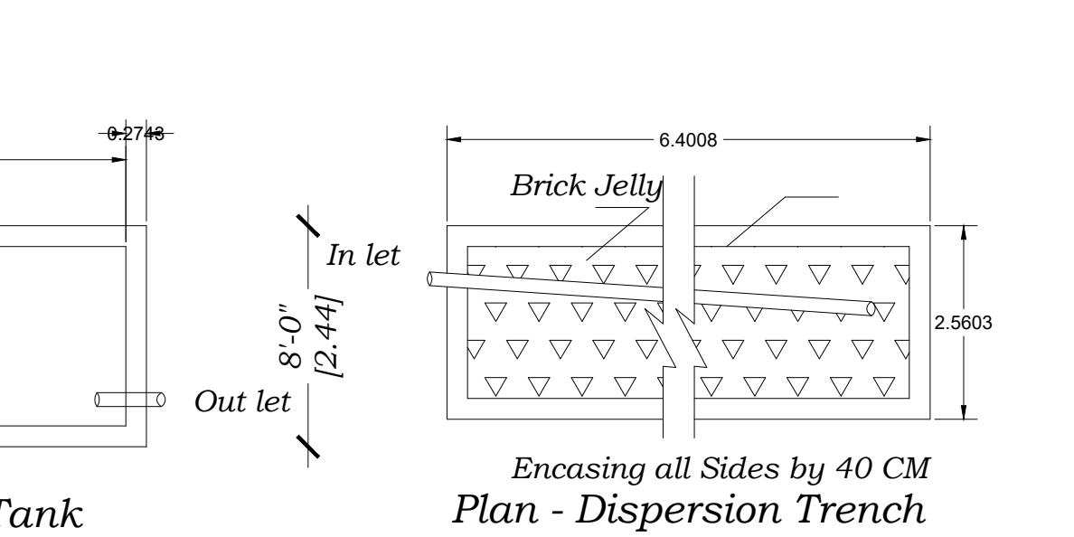
Plan - Dispersion Trench
