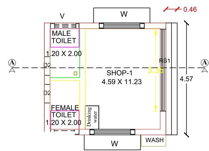
d Ground Floor Plan
