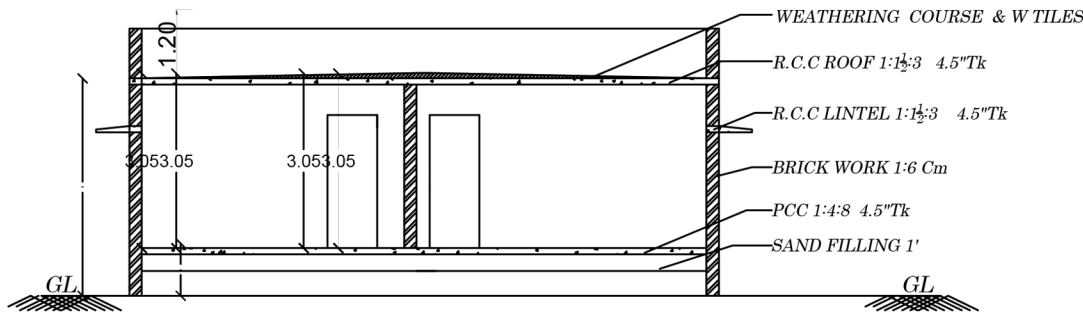
CUT SECTION ON AA
