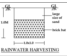
RAINWATER HARVESTING
