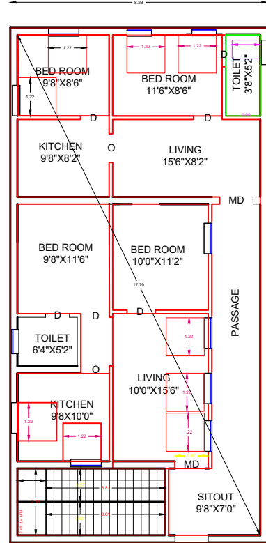
GROUND FLOOR PLAN [EAST FACING]
