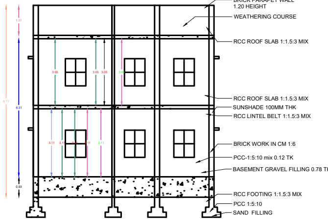
SECTION
