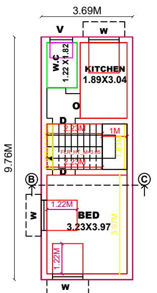
PROPOSED SECOND FLOOR PLAN (RESIDENTIAL)
