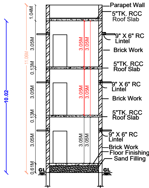
SECTION ON "BC"
