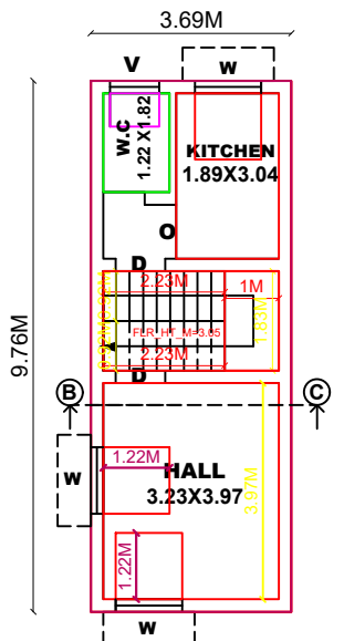
PROPOSED FIRST FLOOR PLAN (RESIDENTIAL)
