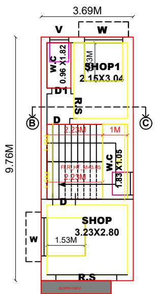
EXISTING GROUND FLOOR PLAN (COMMERCIAL)
