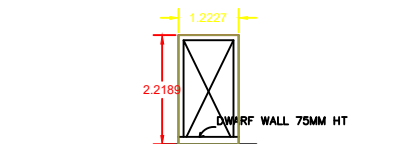
WICKET GATE
