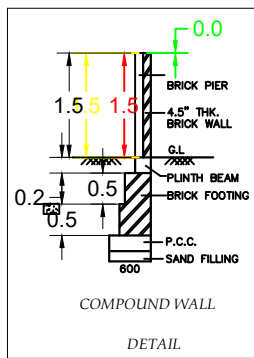
DETAIL
