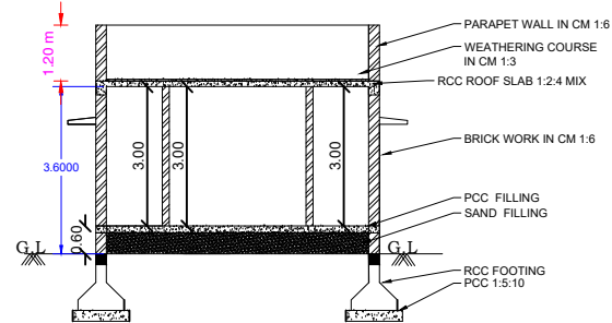
SECTION-"SR"
