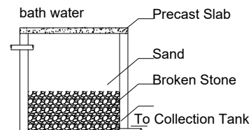
Section of Filter Unit
