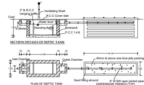
DETAILS OF SEPTIC TANK & DISPERSION TRENCH
