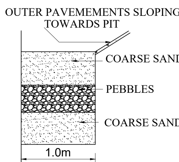
RAIN WATER PERCOLATION BED
