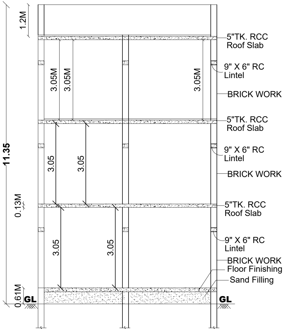
SECTION ON S-R
