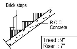
STAIRCASE DETAILS
