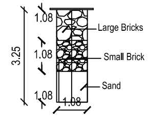
SECTION OF RAIN WATER
