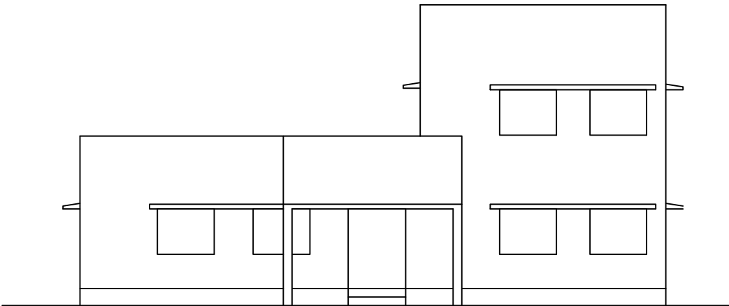
FRONT ELEVATION (EAST FACING)
