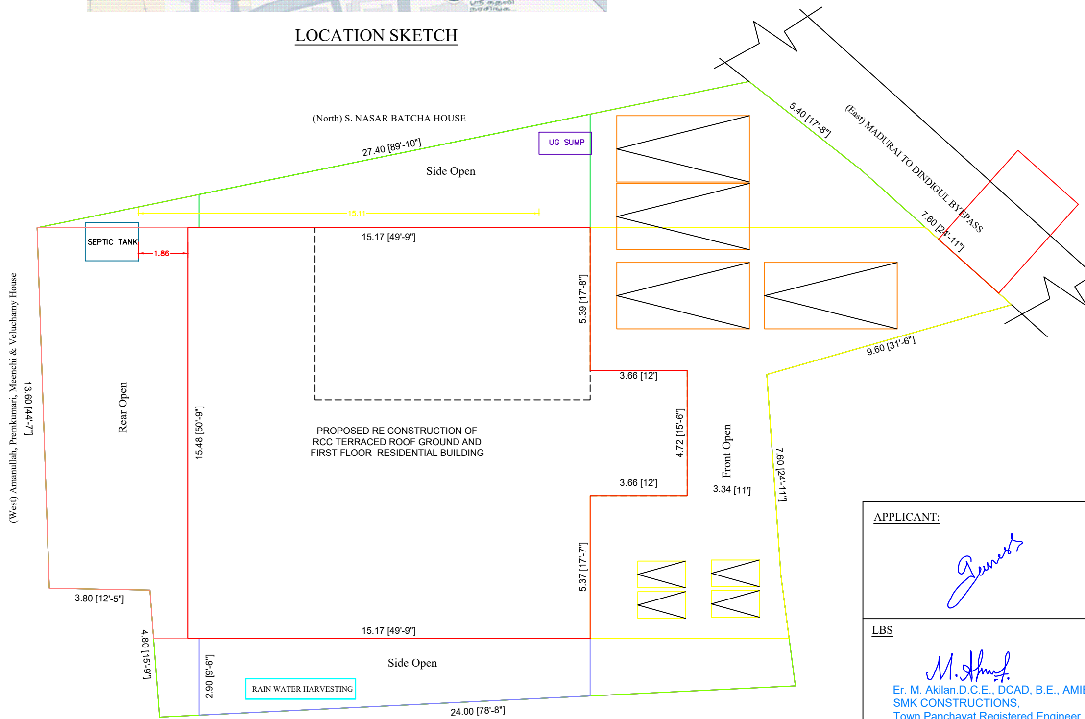
SITE PLAN
