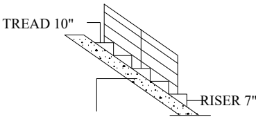
STAIRCASE DETAILS [N.T.S.]
