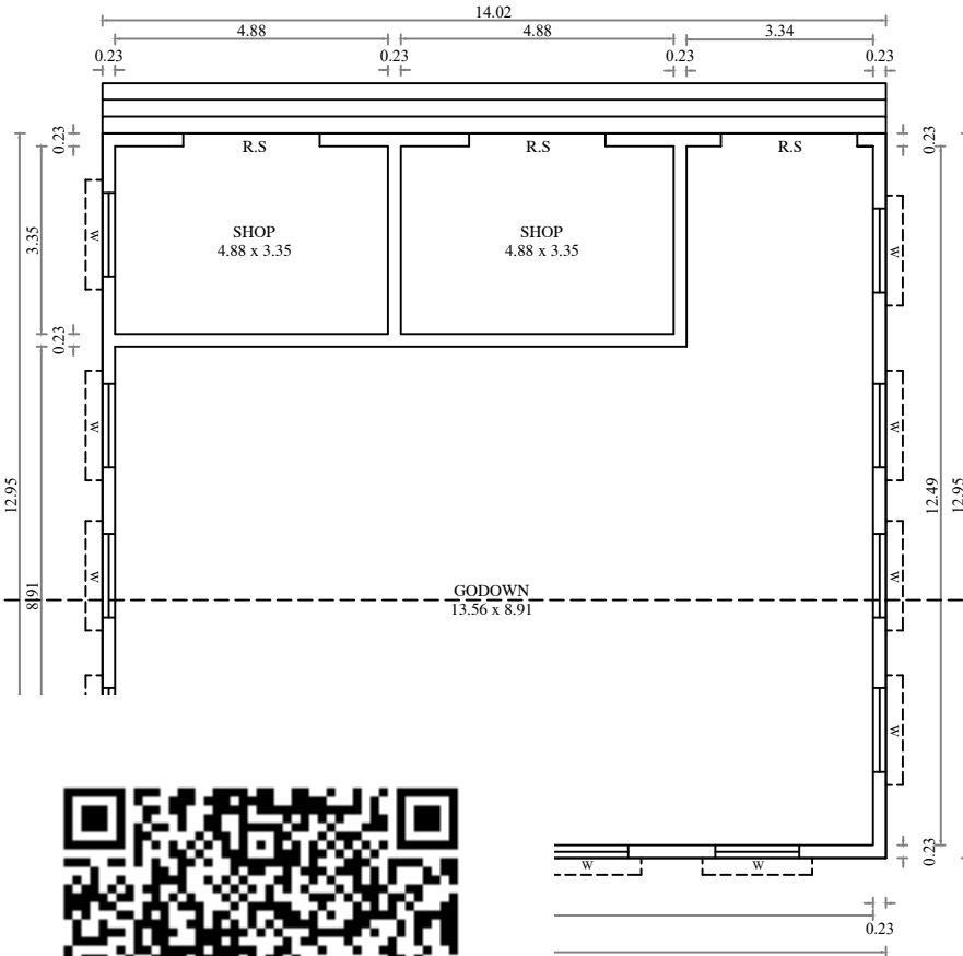
FLOOR
