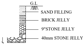
RAIN WATER HARVESTING RECHARGE PIT
