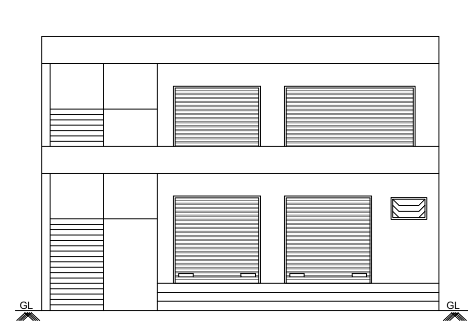
FRONT ELEVATION (EAST FACING)
