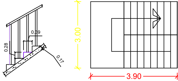
STAIRCASE DETAILS
