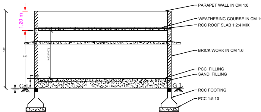
SECTION ON - "SR"
