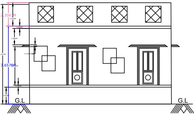
FRONT ELEVATION
