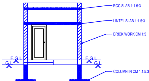
EB SECTION
