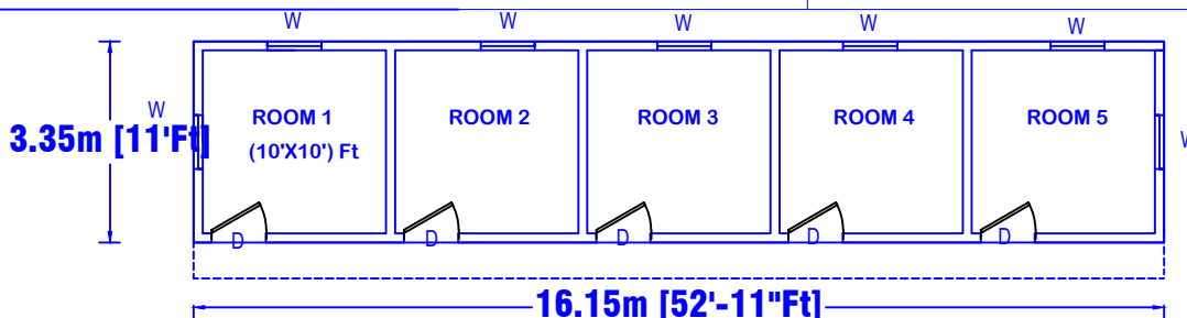
LABOUR SHED PLAN
