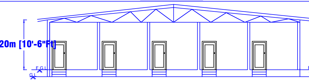
LABOUR SHED ELEVATION
