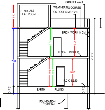
SECTION "A-B"
