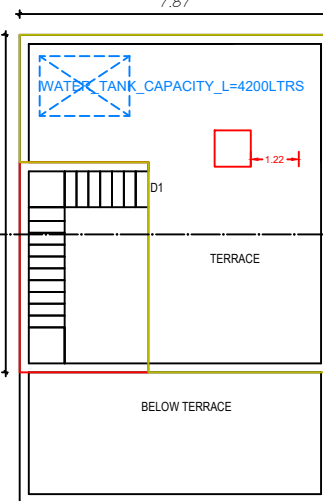
PRO. FIRST FLOOR PLAN.
