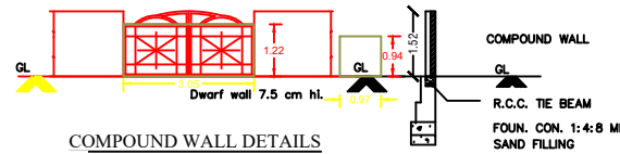
SECTION
