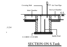
SECTION ON S.Tank
