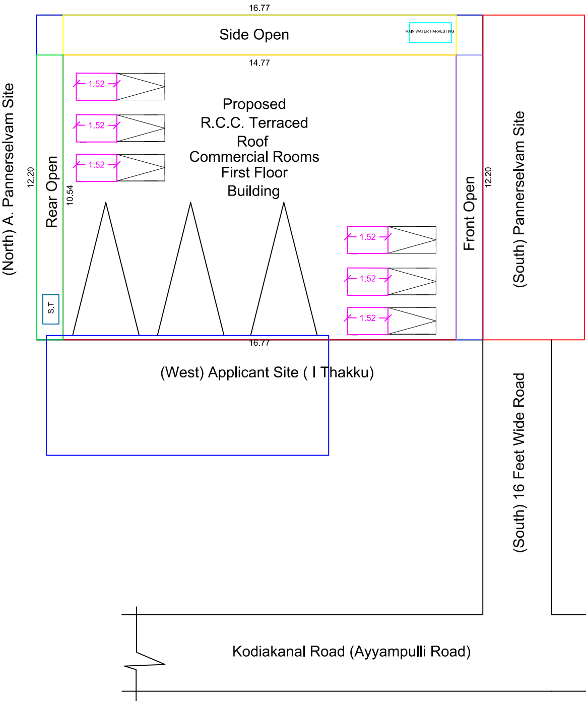
SITE PLAN
