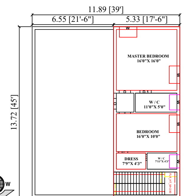
PRO.FIRST FLOOR
