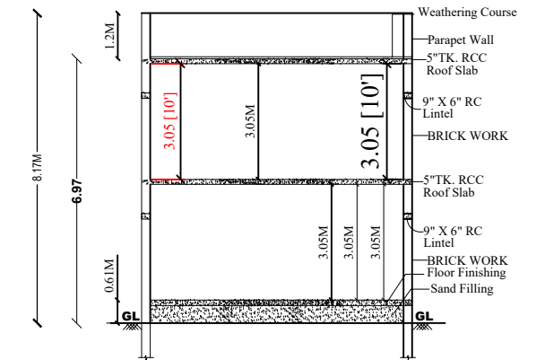
SECTION ON "SR"
