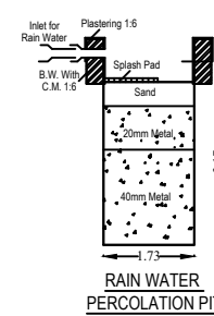
RAIN WATER PERCOLATION PI
