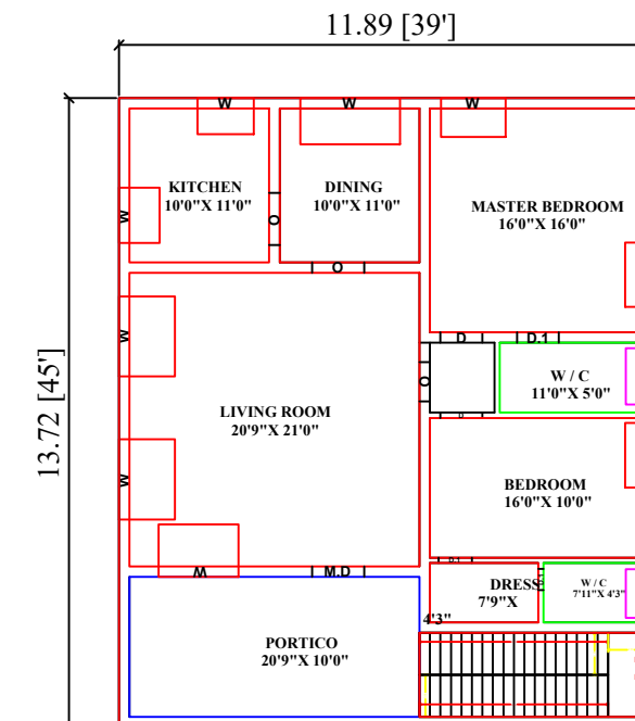
PRO.GROUND FLOOR
