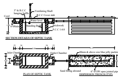
DETAILS OF SEPTIC TANK & DISPERSION TRENCH
