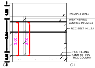
SECTION ON-'AB'
