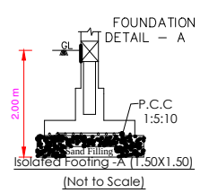
FOUNDATION DETAIL - A
