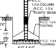
FOUNDATION DETAIL
